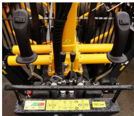
Valve block 4/8 XY control ON-OFF
