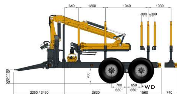
TRAILER 346Re | FW | 710/40-22,5 | Ø 1170
