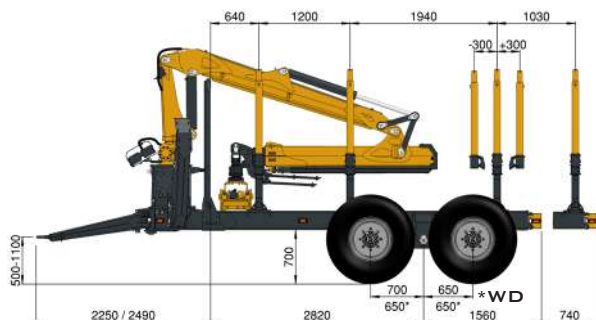
TRAILER 346R | FW | 600/50-22,5 | Ø 1170
